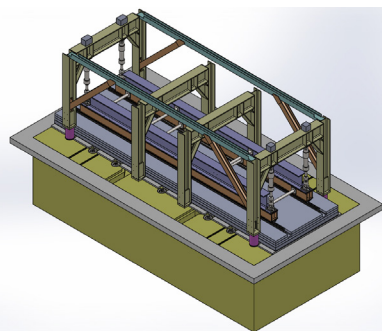
▲ Dynamic loading device SysIFE.
