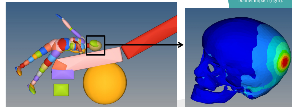
▼ Overall simulation of the accident (left) and local simulation of the head/bonnet impact (right).
